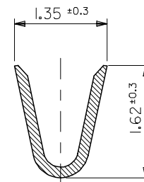
SECT. B-B
