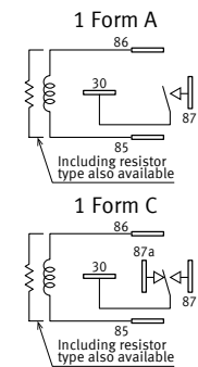
Schematic (BOTTOM VIEW)
