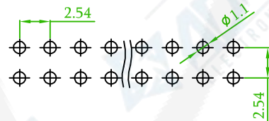
Recommended PCB Layout (PCB TOLERANCE ±0.1)
