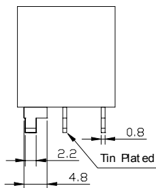
FRC7N - PCB type
