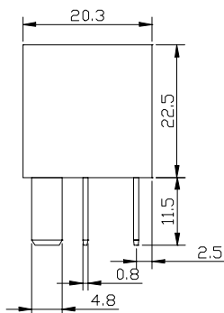
FRC7N - PCB type
